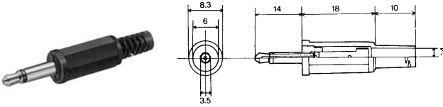
No.MP-106LC (3.5 -2極) 2-CONDUCTOR MINIATURE PLUG w/shielded handle MONO
