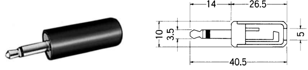
No.MP-105LC (3.5 -2極) 2-CONDUCTOR MINIATURE PLUG MONO
