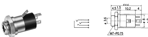
No.MJ-079 (3.5 -4極) 4-CONDUCTOR MINIATURE JACK
