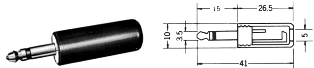
No.MP-105L (3.5 -2極) 2-CONDUCTOR MINIATURE PLUG. MONO
