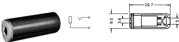
No.MJ-164 (3.5 -2極) MINIATURE INLINE JACK MONO
