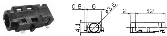
No.M03-992C0 (3.5 -4極) 4-CONDUCTOR MINIATURE JACK FOR P.C.B
