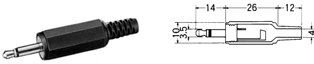
No.MP-104MH (3.5 -2極) 2-CONDUCTOR MINIATURE PLUG MONO
