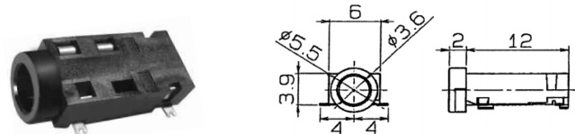
No.M03-992C0 (3.5 -4極) 4-CONDUCTOR MINIATURE JACK FOR P.C.B
